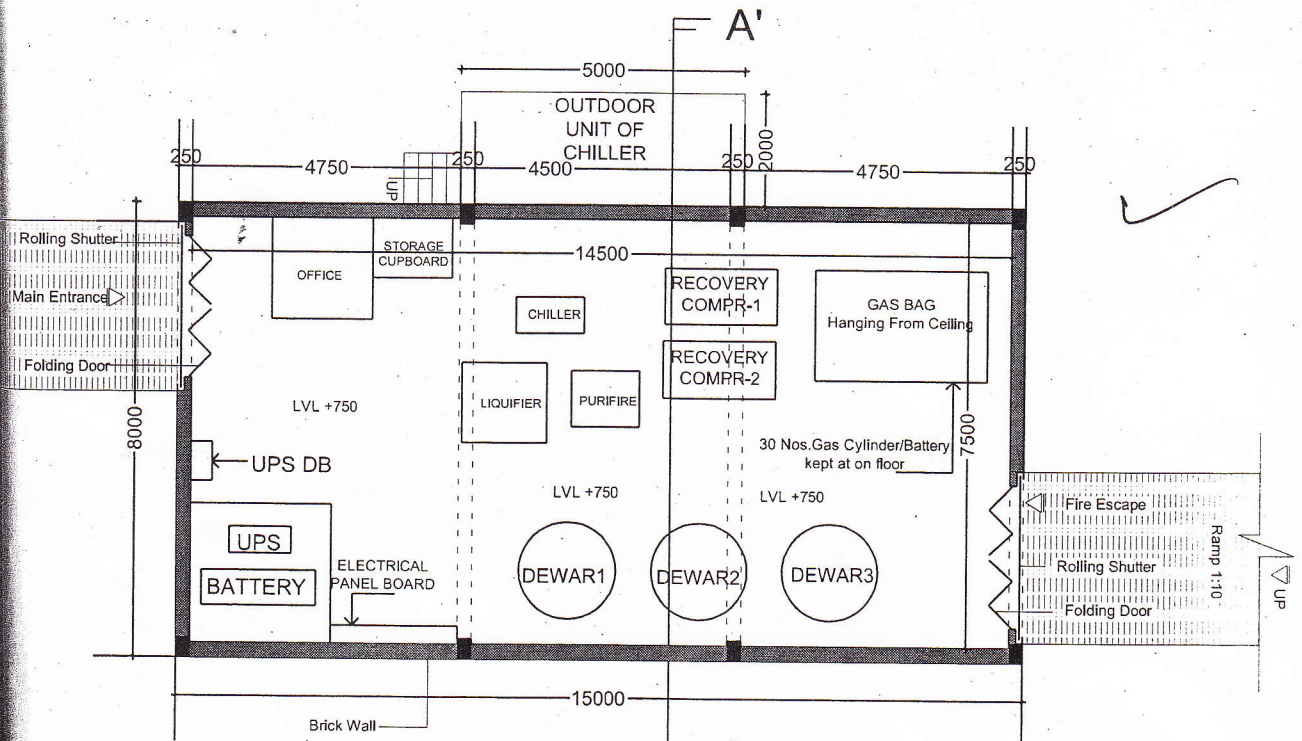
GROUND FLOOR PLAN ( BELOW LVL +1750 )
