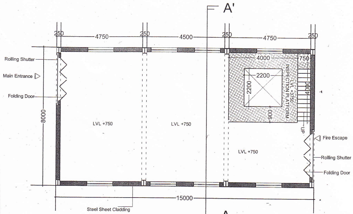
GROUND FLOOR PLAN ( ABOVE LVL +1750 )
